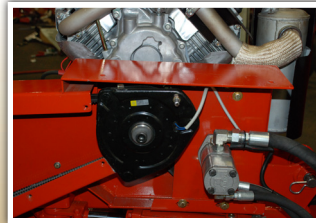
ELECTRIC CLUTCH Electric clutch cutter head engagement with electronic shut-down brake
